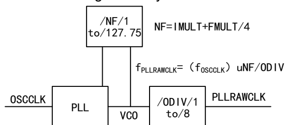
Figure 20 System PLL
