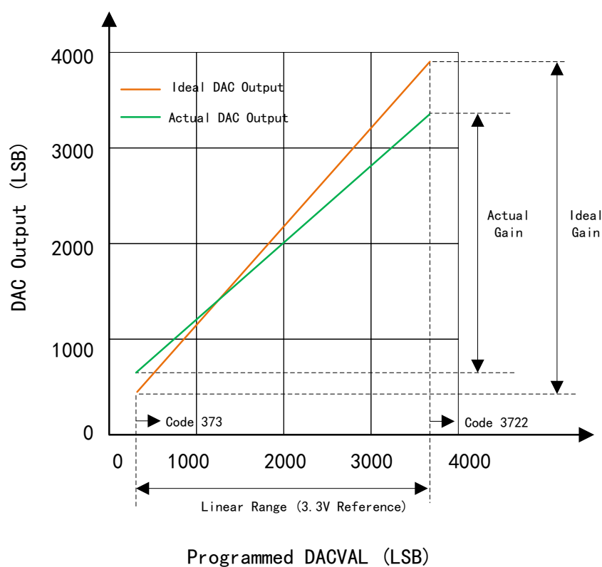
Figure 49 Linearity of Buffer DAC
