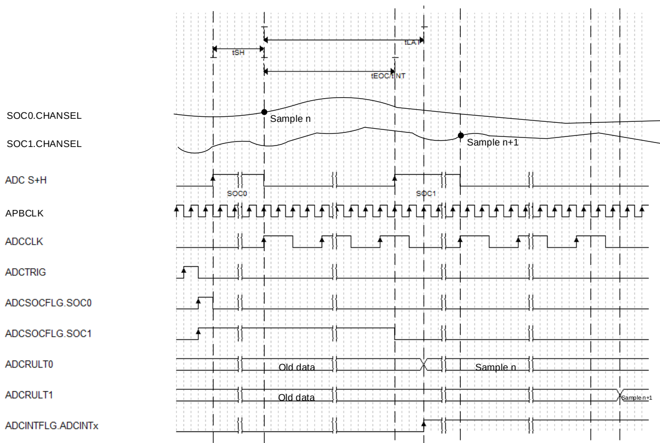
Figure 45 ADC Timing
